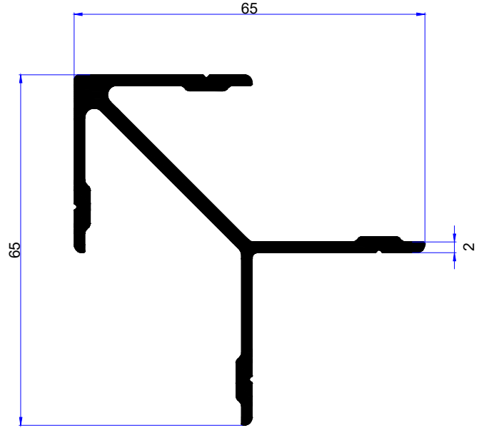
PROFİL KODU / PROFILE CODE 2664 AĞIRLIK / WEIGHT 1,081 GR/M
